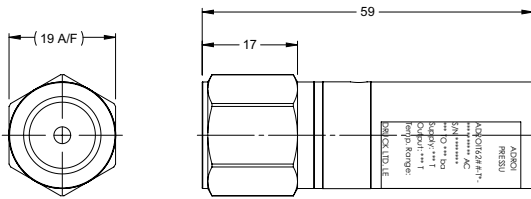
LOW PRESSURE CONSTRUCTION (PRESSURE RANGES: <10 bar)
